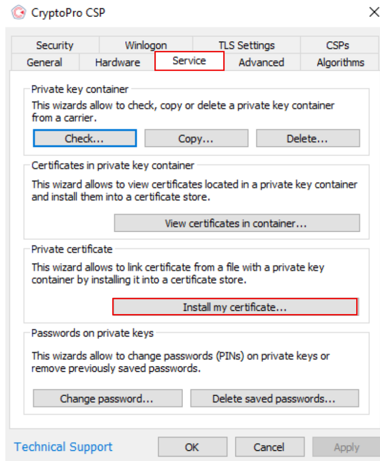
Figure 1 – "Service" tab with the "Install my certificate..." button.
