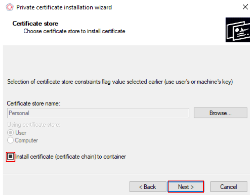
Figure 6 - Certificate Store selection screen with "Personal" store selected and "Install certificate into the container".
